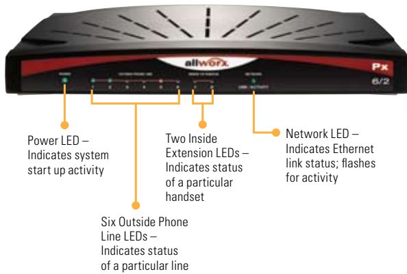
Figure 1: Front View
