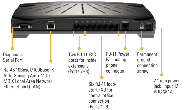
Figure 2: Rear View
